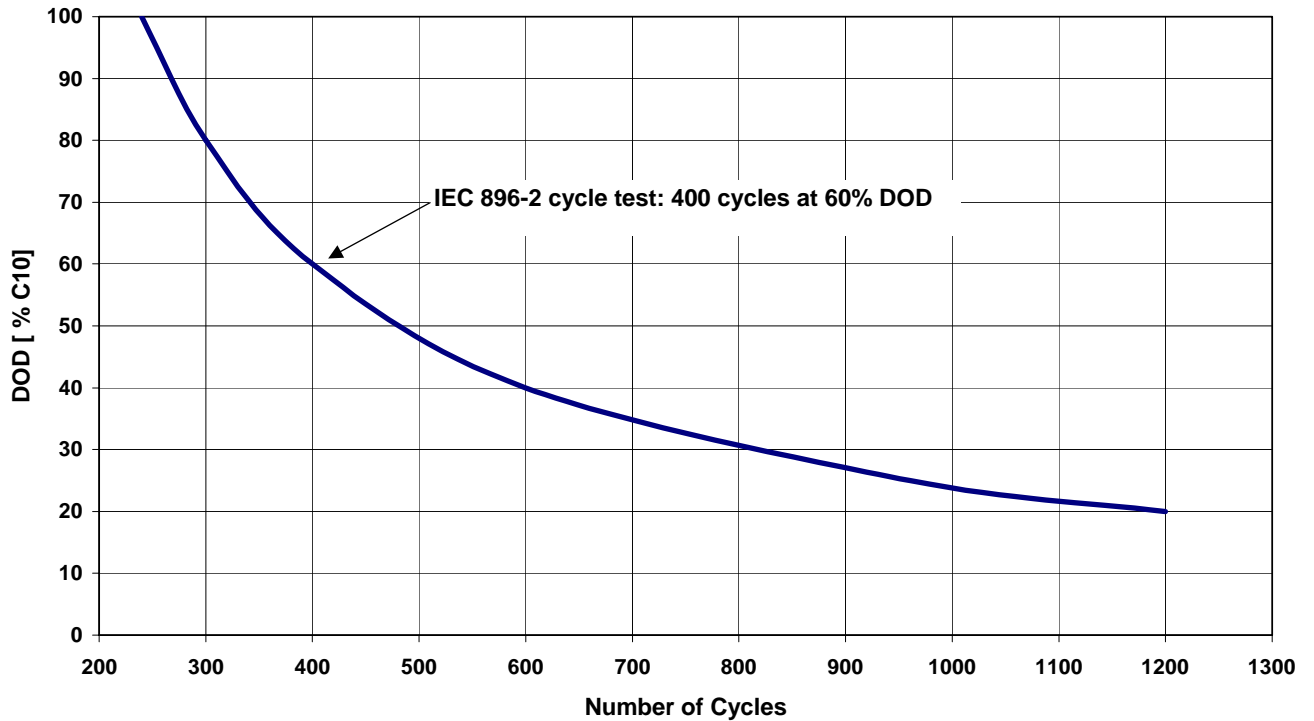
Fig. 10: Marathon - Number of Cycles vs. Depth of Discharge (DOD)
