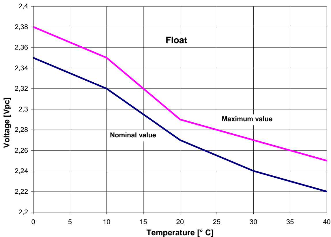
Fig. 5: Marathon L, Powerfit S – Charging Voltage vs. Temperature. The charging voltage must be set to the nominal value. The maximum value must not be exceeded.
