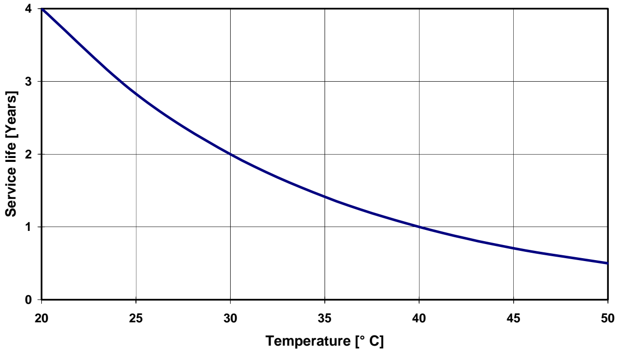
Fig. 15: Powerfit S 300 - Service Life vs. Temperature
