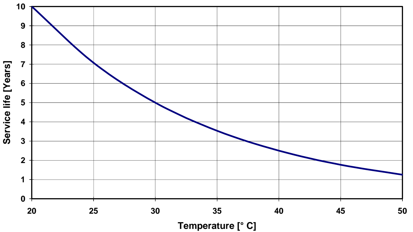
Fig. 18: Marathon – Service Life vs. Temperature
