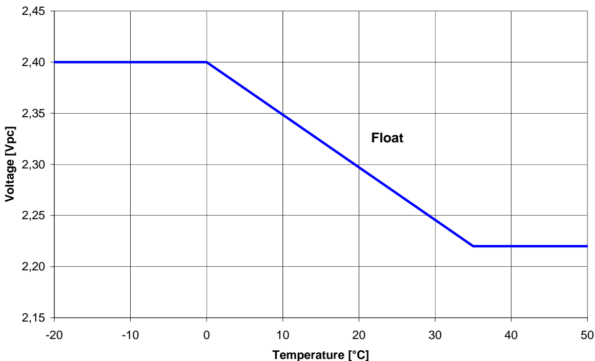
Fig. 6: Marathon M, Sprinter P and S – Charging Voltage vs. Temperature
