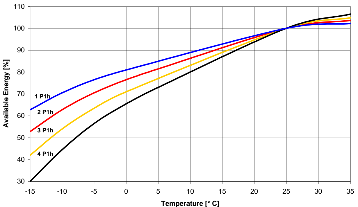
Fig. 14: Sprinter – Available Energy vs. Temperature at different Discharge Rates (multiples of the 1-hour-power)
