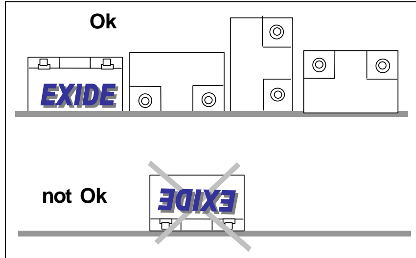
Fig. 3: Installation positions for AGM-blocks.
