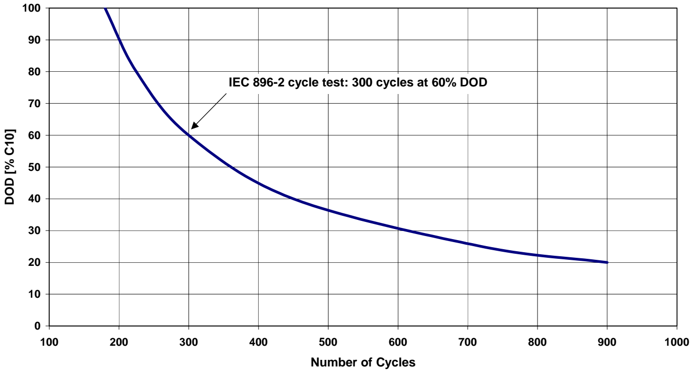
Fig. 9: Sprinter, Powerfit – Number of Cycles vs. Depth of Discharge (DOD)
