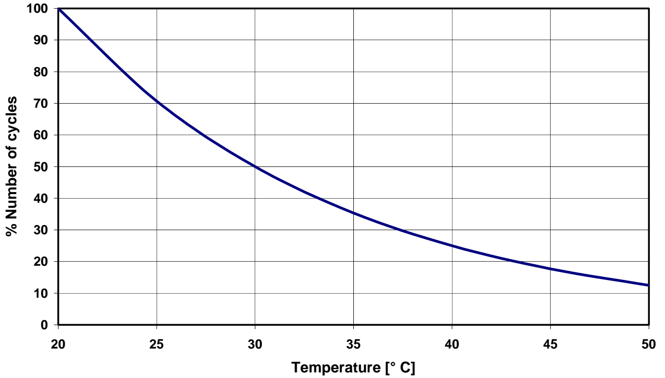
Fig. 19: Endurance in Cycles (in % of number of cycles) vs. Temperature
